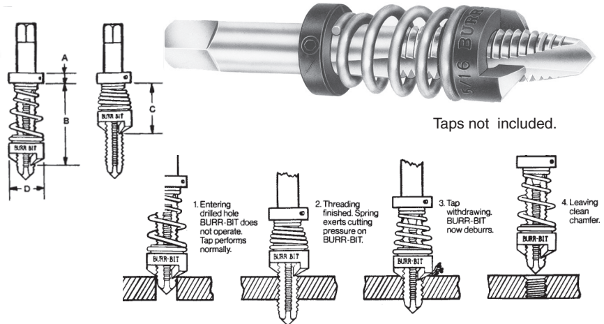
BURR-BITS FOR TWO & FOUR FLUTE TAPS - INCH & METRIC
